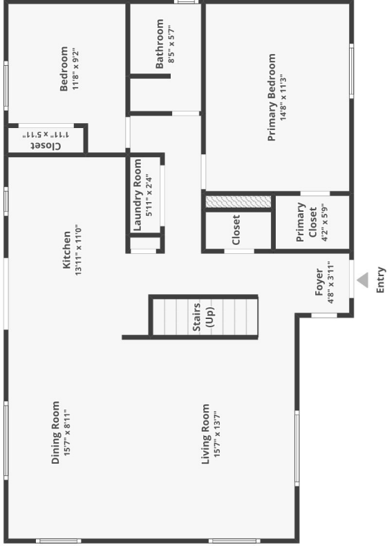
FLOOR 1
